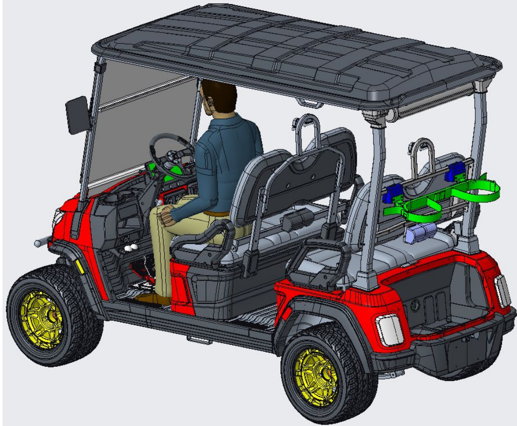
Install Golf Bag Bracket
